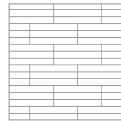
B-strip, brickbond
